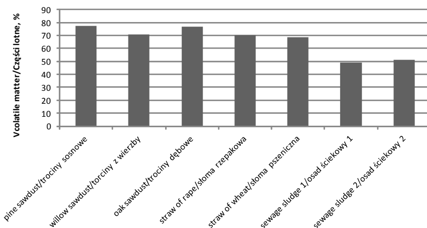
Fig. 3. Volatile matter content of analysed feedstock
