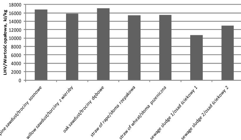
Fig. 2. Lower heating value of analysed feedstock
