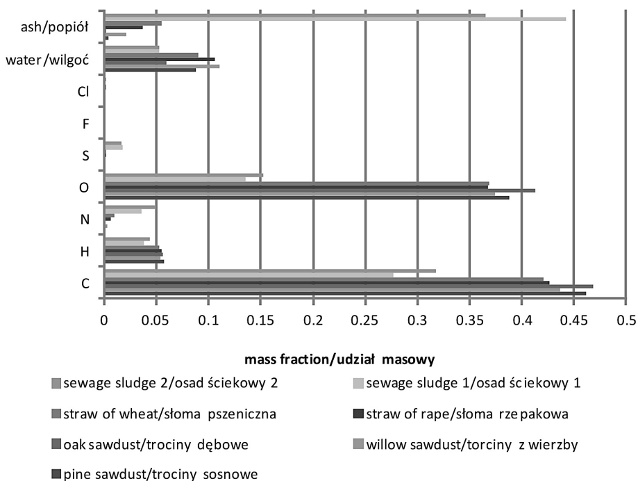
Fig. 1. Ultimate analysis and ash and water content in analysed feedstock
